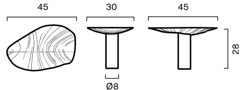
VALE knob oval 45 mm
